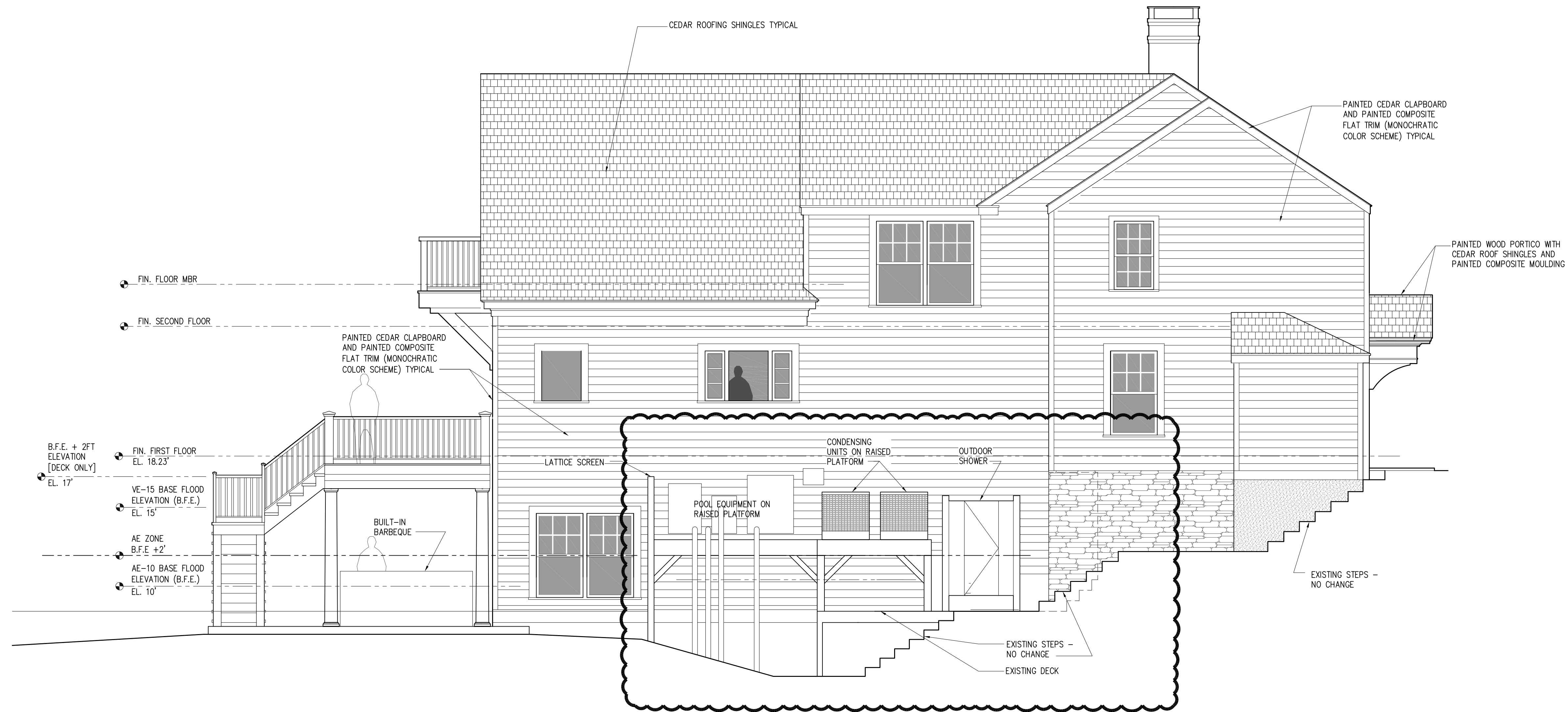
2 BUILDING ELEVATION (WEST) SCALE: 1/4"=1'-0"
